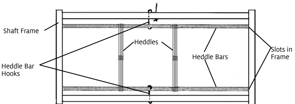
FIGURE 3: SHAFTS / HEDDLES
